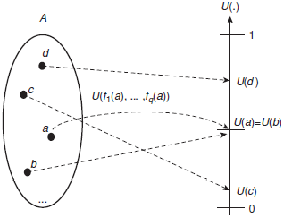
Figure 1: Representation of the ranking of the set A using the MAUT model [17].
